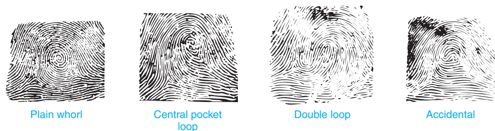
FIGURE 14-6 Whorl patterns.
